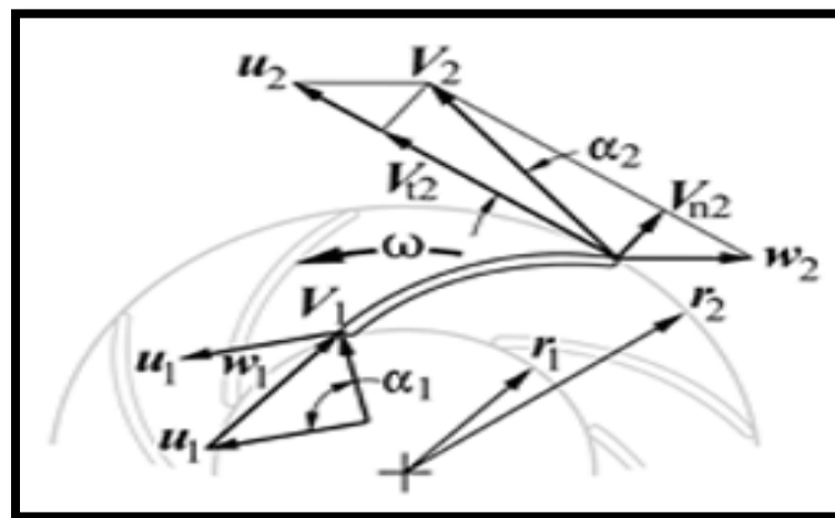
Figure 2.2. Centrifugal impeller velocity triangle
