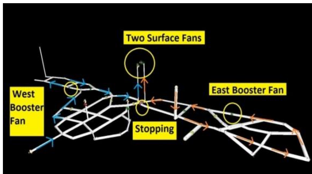
Figure 4.7. Experimental Mine Ventsim Visual, Model- scenario 1
